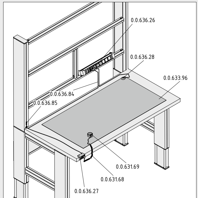
Illustration of an ESD-safe work bench.
